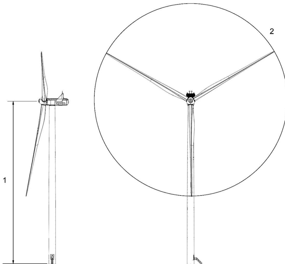
Figure 3-1: Illustration of outer dimensions – structure
